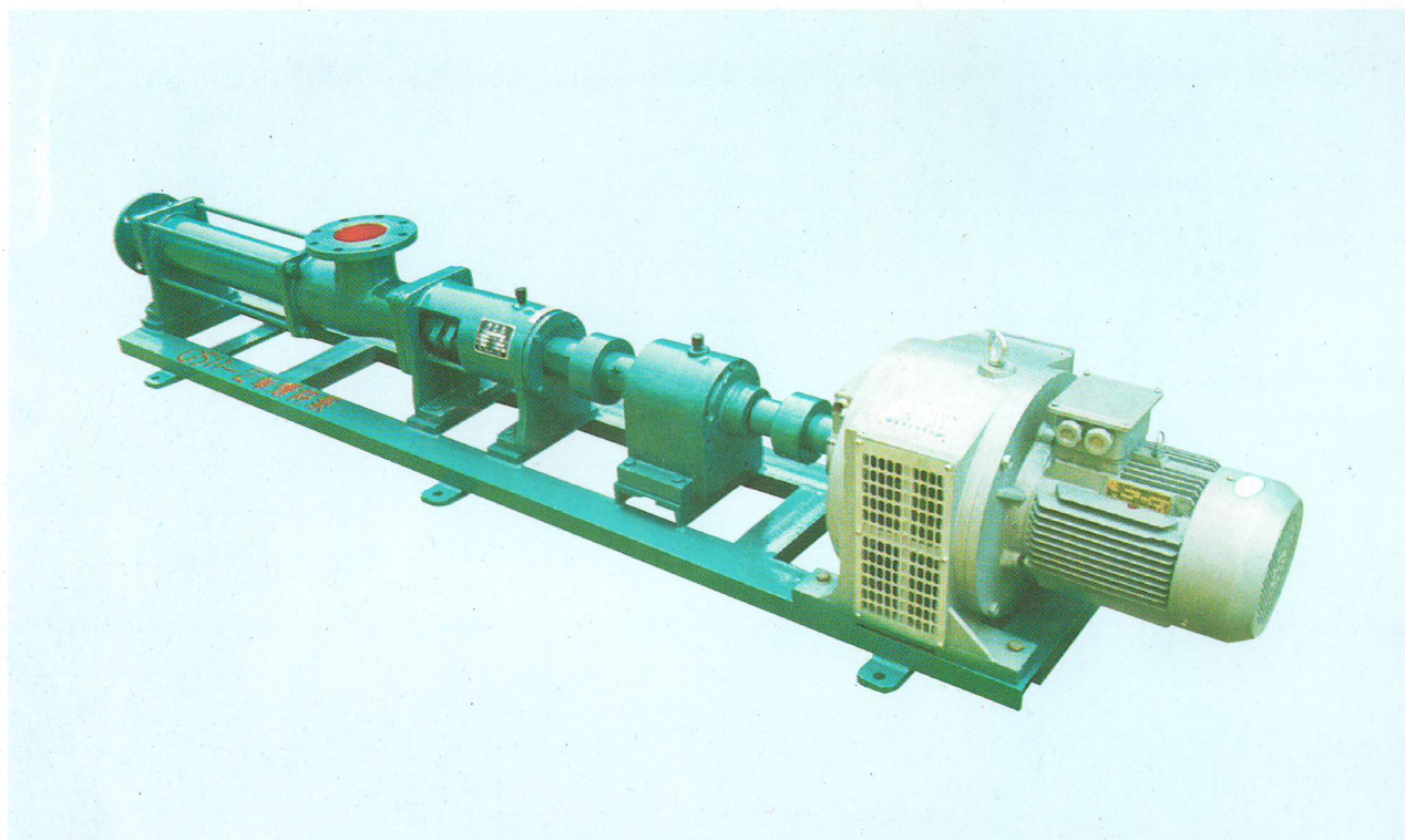
G TYPE SCREW PUMP
